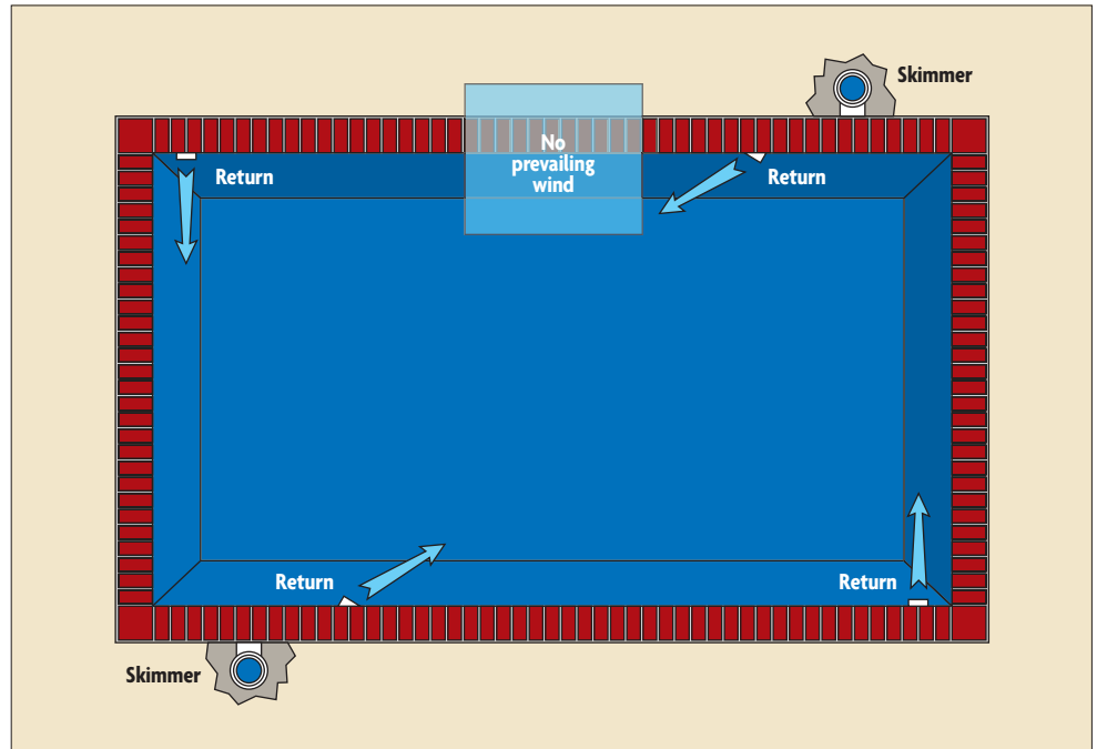
A no-drainer: In a pool without a main drain, skimmers should be placed to accommodate wind direction and/or flow pattern (below). In all cases, position the returns to move the water so it passes in front of skimmer openings at a moderate speed. No returns should move the water to the skimmers closer than 10 feet from the openings. Locate returns so they move water at the surface and near the bottom.
