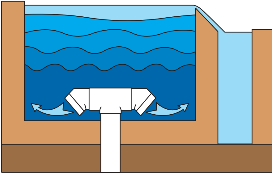
Calm source pool: A smooth water surface in the upper pool helps control the waterfall flowing into the lower pool. Attach a tee and elbow fittings to the feed pipe. This contains motion by splitting the water and pointing it toward the floor.
